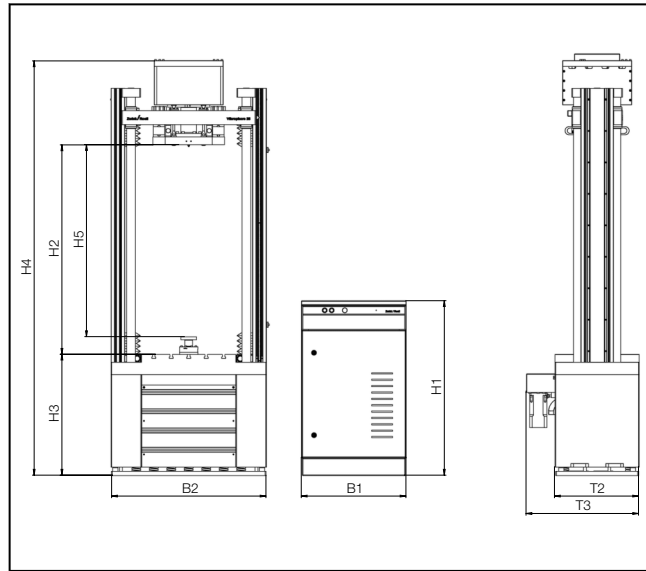
Drawing: Vibrophore 25
